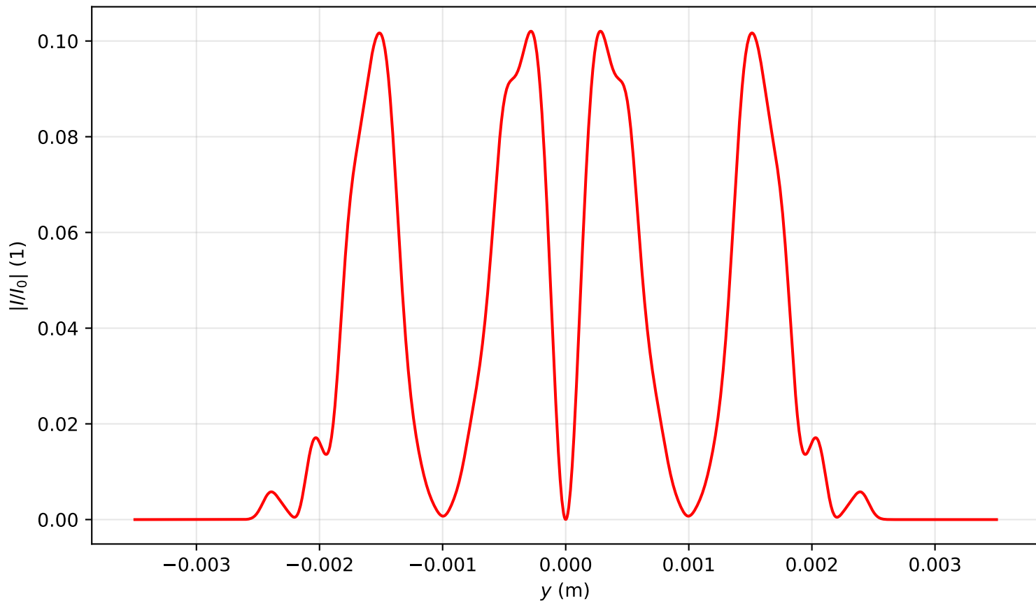
Intensity profile I(x=0, y, z=2.388)/I_0 , P_{in}=9.0P_{cr} , artificial time
